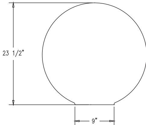
ELEVATION VIEW
