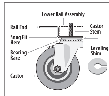
Fig. 7. Castor diagram.
