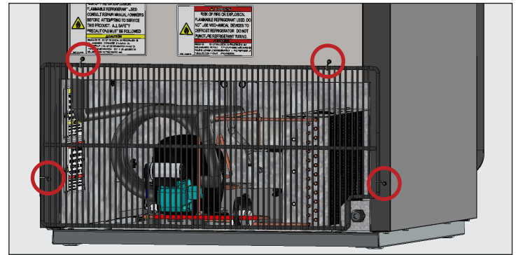
Fig. 2. CVM-27 rear grill screw locations.
