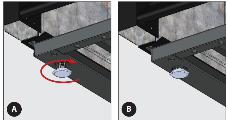
Fig. 2. Turn the leveling screws clockwise to lower the unit.
