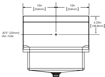
■ Hole Configuration
