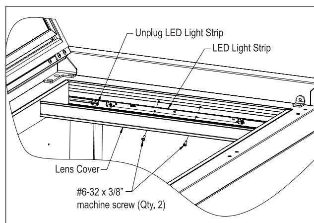
Figure 15: Interior LED Light
