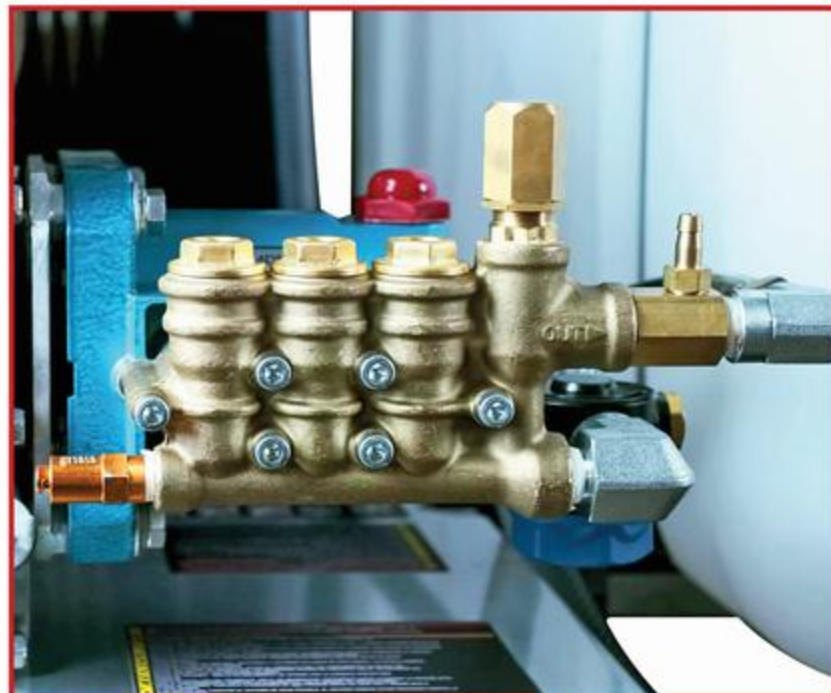
CAT PUMPS® Triplex integrated unloader for easy pump maintenance
