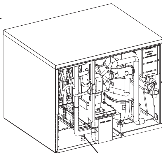
Fig. 10 Drain Plug
