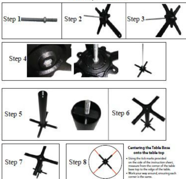
Assembly Illustration
