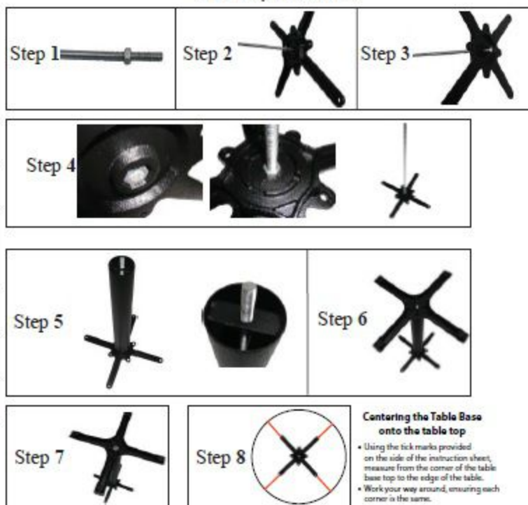
Assembly Illustration
