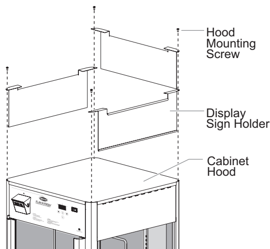
Display Sign Holder Installation
