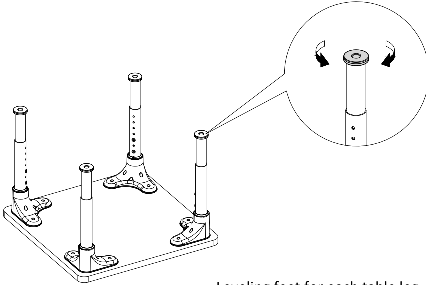
Leveling feet for each table leg
