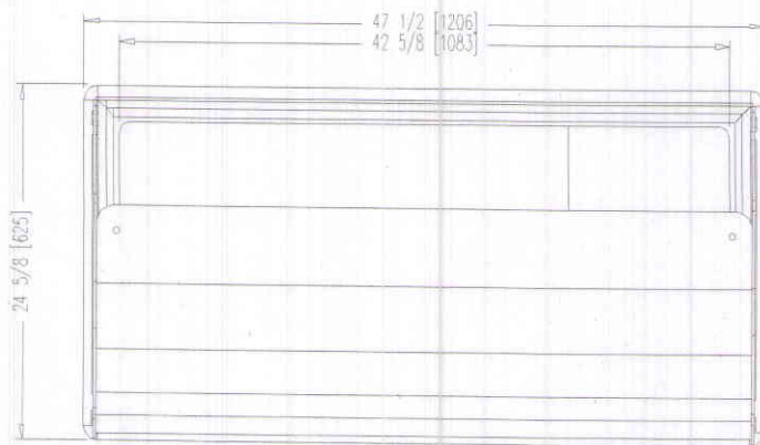
VISTA SUPERIOR Top view
