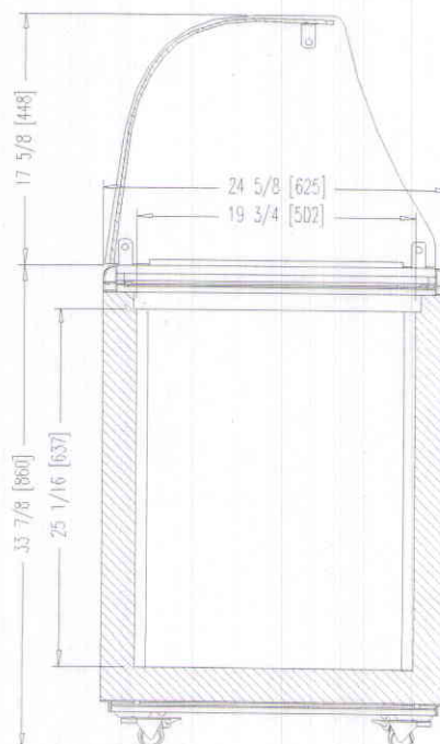
VISTA LATERAL Side view
