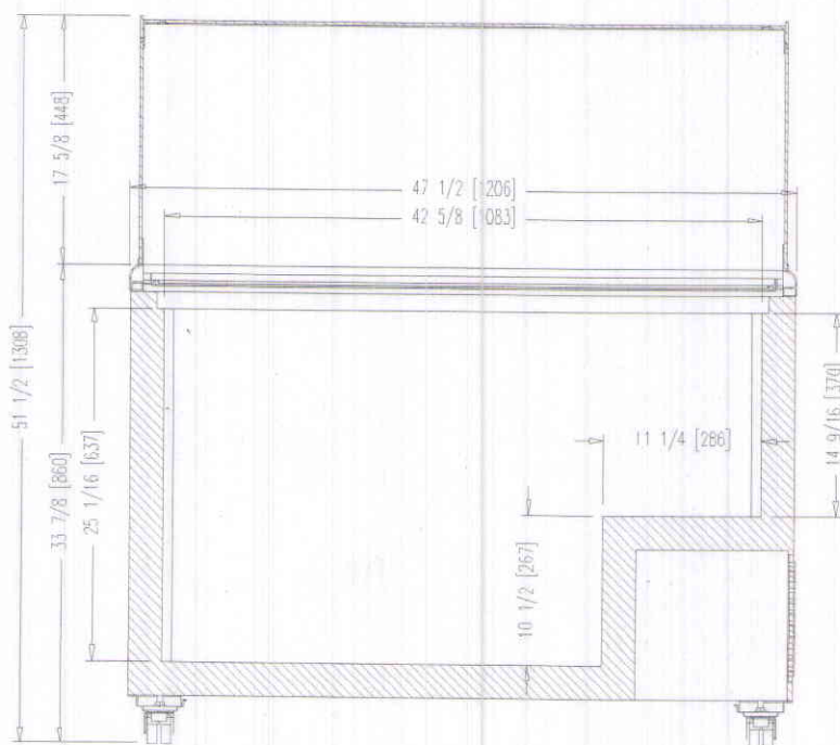
VISTA FRONTAL Front view
