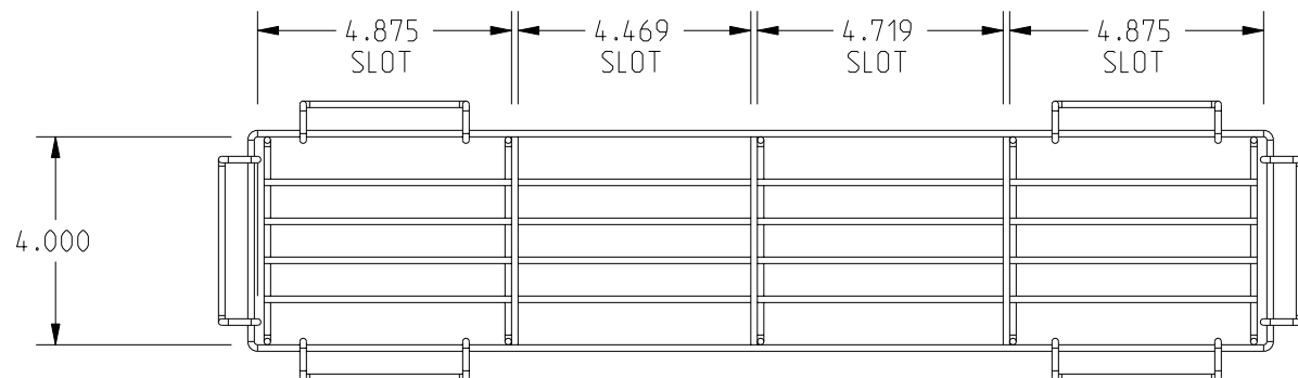
TOP VIEW
