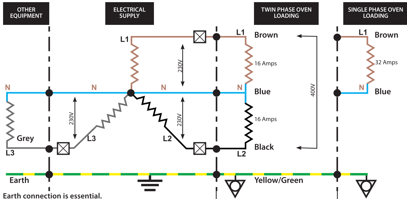
Phase Loading Diagram
