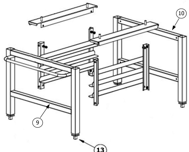
DSK272831 fitted with Adjustable Feet
