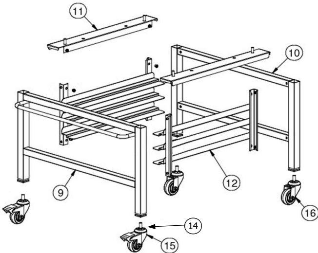
DSK272831C fitted with Castors
