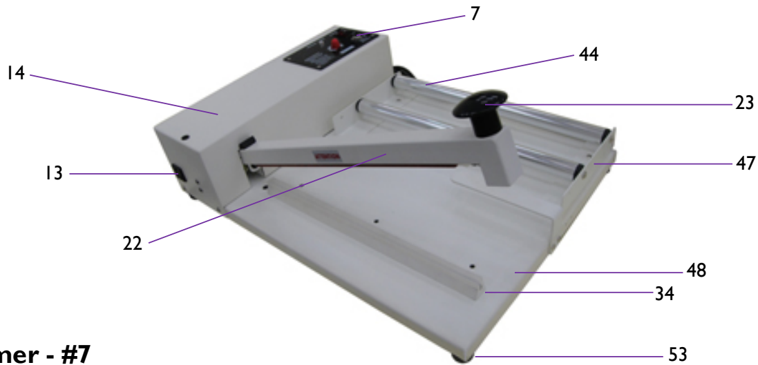
Figure 2. Spare Parts Diagram Overview
