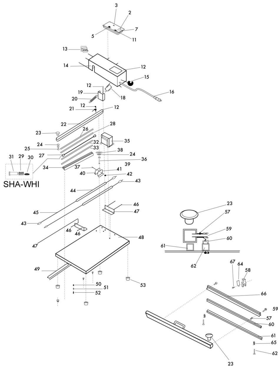
Figure 1. Spare Parts Diagram Overview
