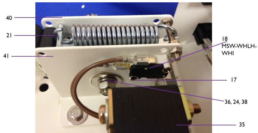
Figure 3. Spare Parts Diagram Overview
