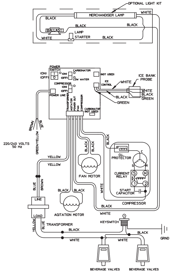
CEV-30 & CEV-40 EXTERNAL CARBONATION & NON-CARBONATED
