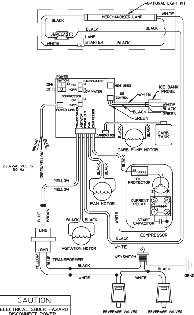
CEV-30 & CEV-40 INTERNAL CARBONATION
