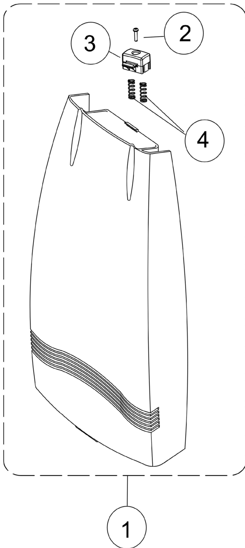
PV130-W14-U Dust Cover Parts
