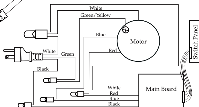
Wiring Diagram
