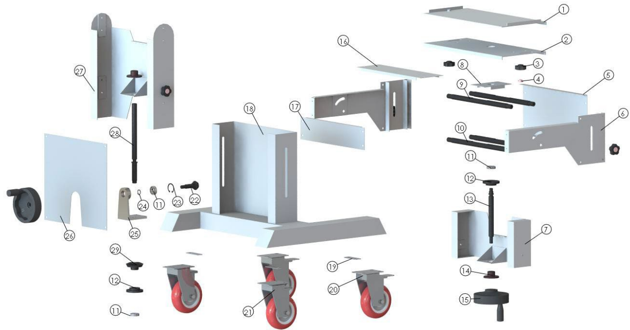
Figure 10. Sealer Rack
