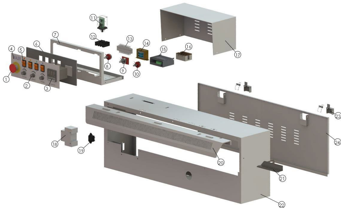
Figure 9. Sealer Head
