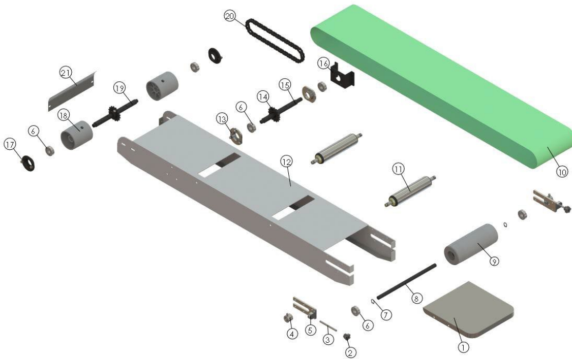
Figure 7. Conveyor
