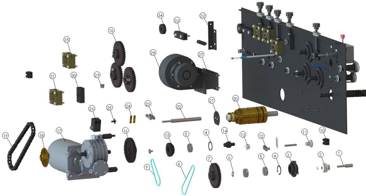
Figure 5. Sealer Gears
