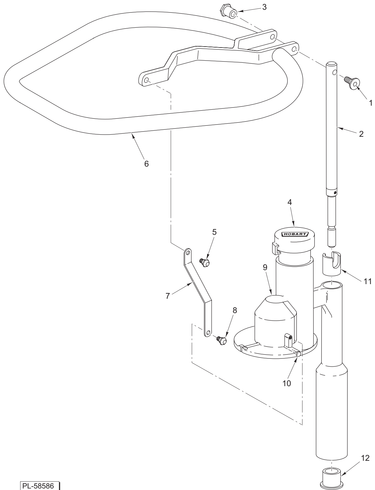
PUSH FEED HANDLE UNIT (ML-136150)
