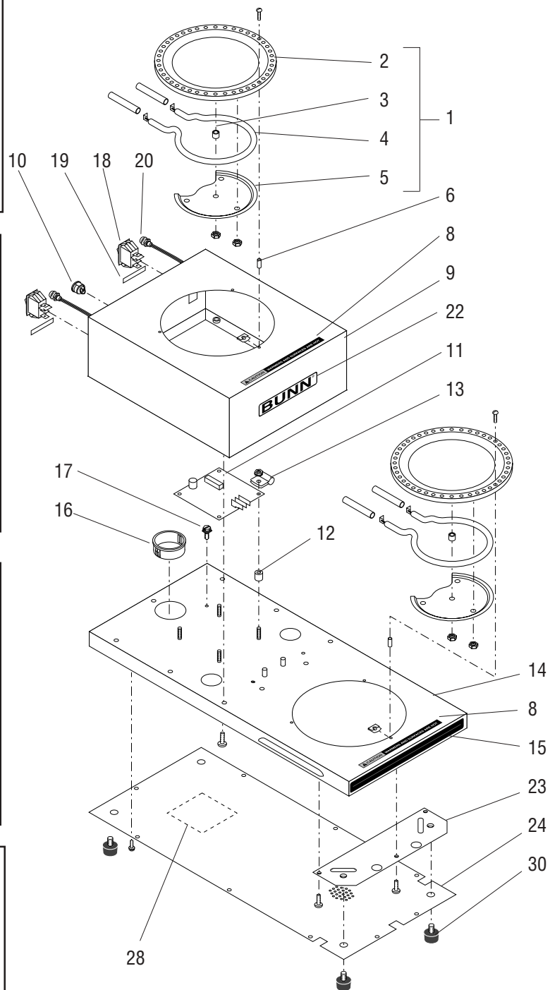
First Type-One Piece Floor Without Adjustable Legs
