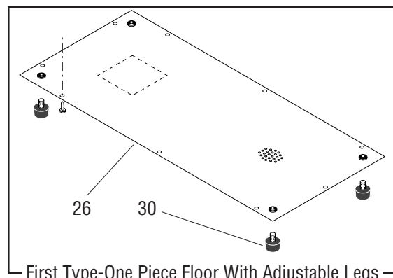
First Type-One Piece Floor With Adjustable Legs
