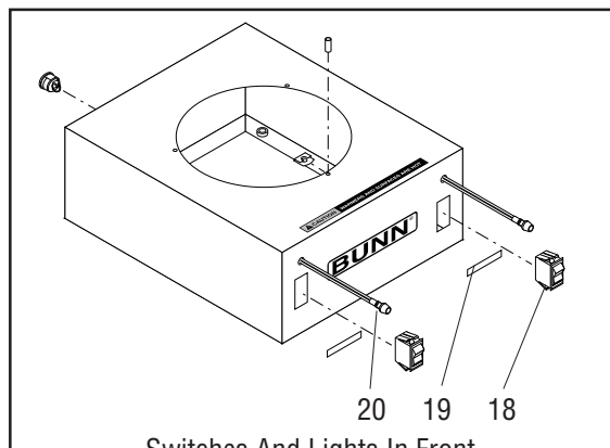
Switches And Lights In Front
