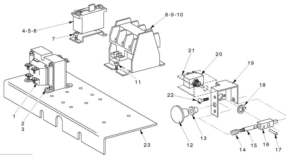
ELECTRICAL UNIT
