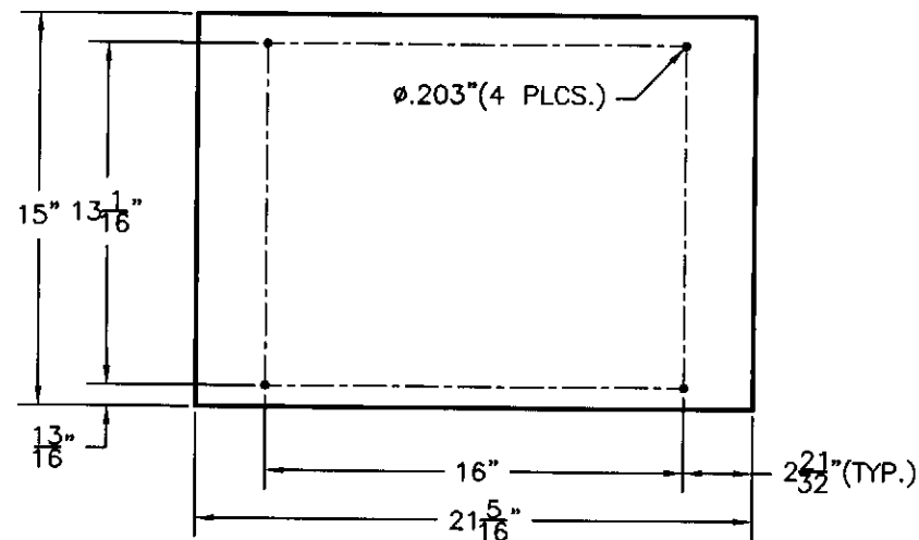
REAR VIEW OF MOUNTING HOLES.
