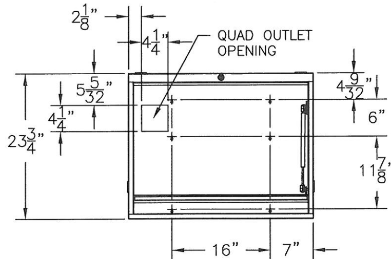
FRONT VIEW (DOOR OPEN)
