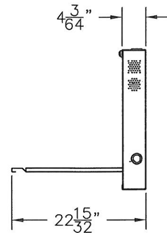
RIGHT SIDE VIEW (DOOR OPEN)
