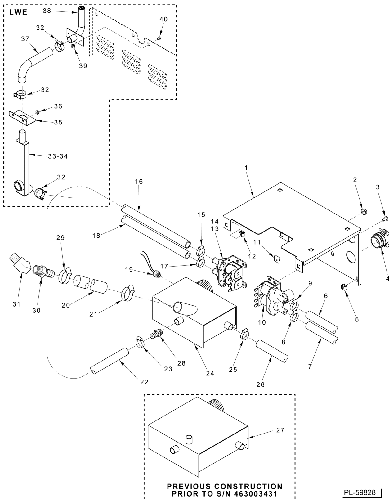
CABINET VALVE
