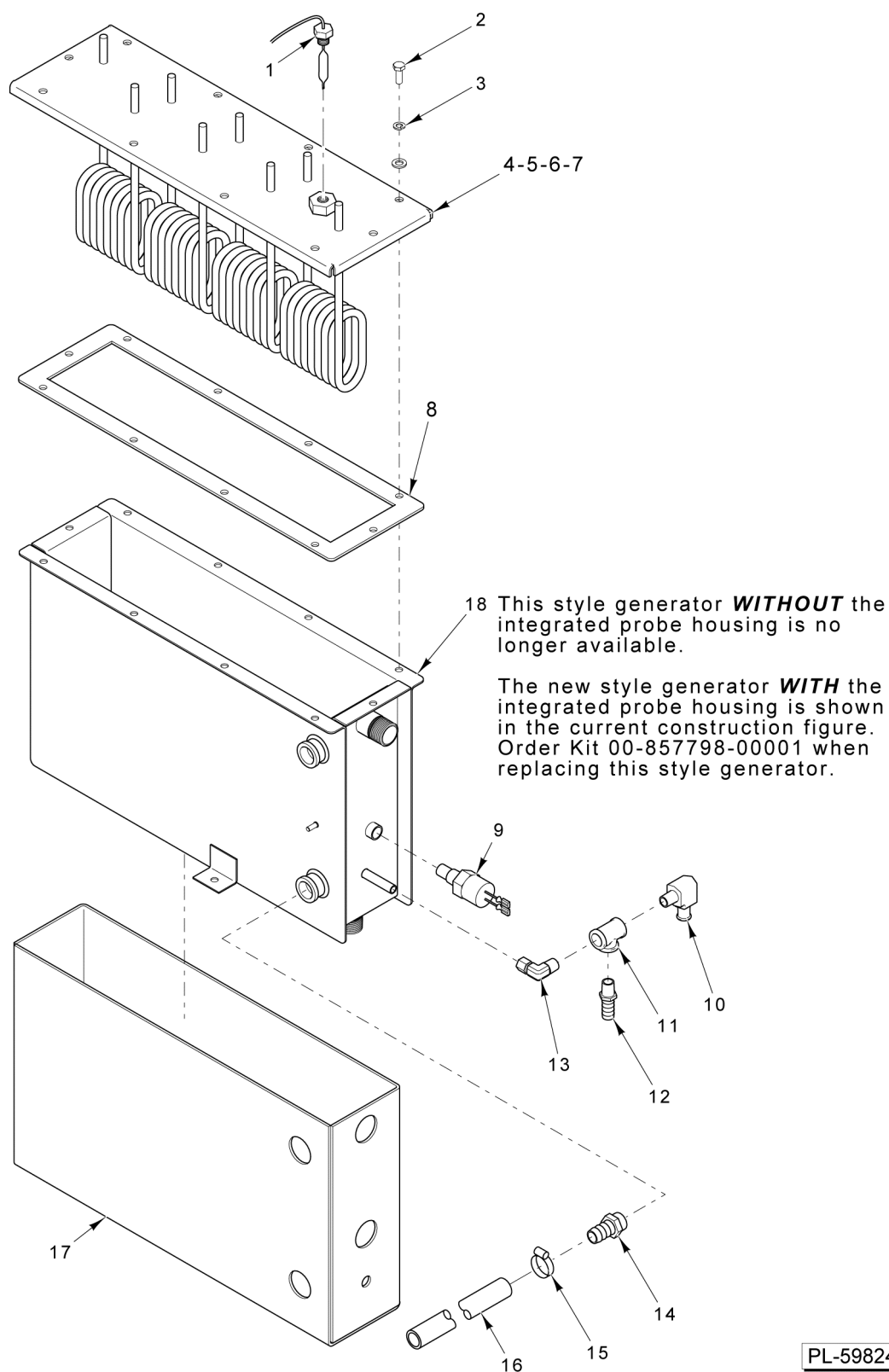
GENERATOR ASSEMBLY (BEFORE S/N 463003747)
