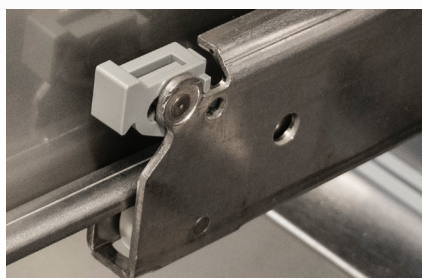
12-GAUGE DRAWER SLIDES with 3 Delrin encased stainless steel roller bearings per each drawer slide
