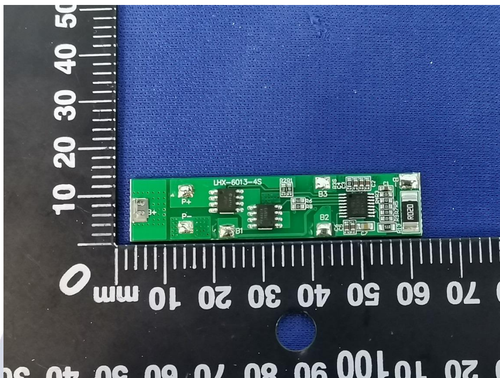
Picture 5. Front view of Protection board-1 图片 5. 保护板前视图-1
