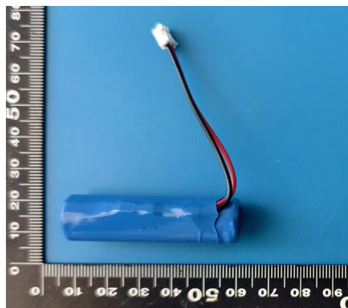
Fig. 2 – Back view of Battery 表2-电池反面视图
