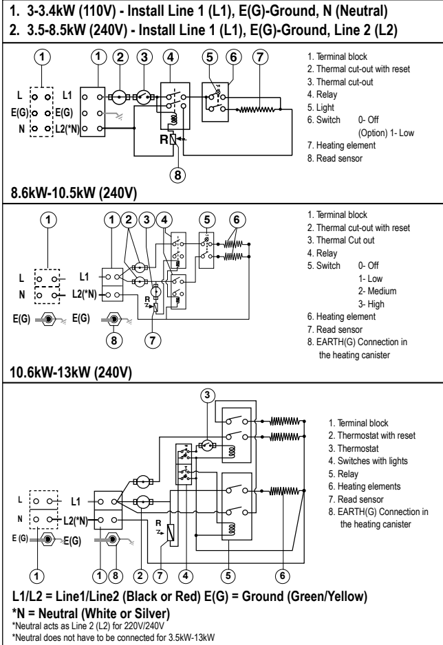
Figure 10 - Water Heater Wiring
