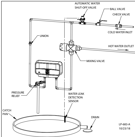
Figure 8 - Installation Detail
