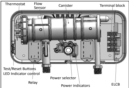
Figure 6 - Water Heater Component Detail
