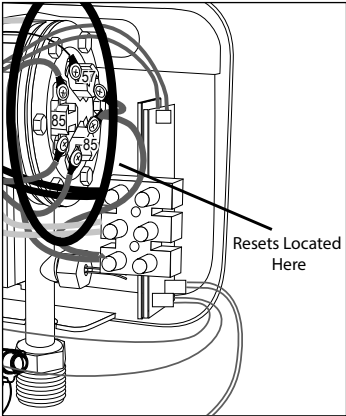
Figure 12 - Reset Locations
