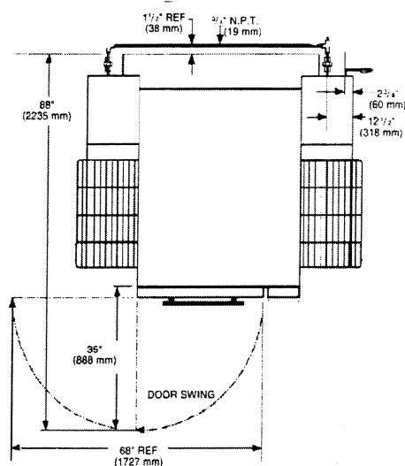
TOP VIEW ELECTRIC
