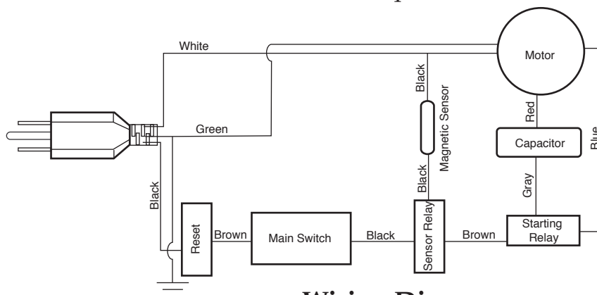
Wiring Diagram
