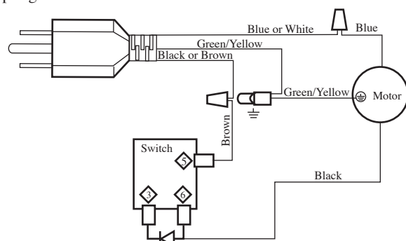
Wiring Diagram for Stainless Steel Top Housing (current production)
