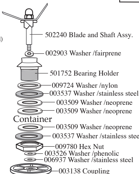
501832 Blending Assy.
