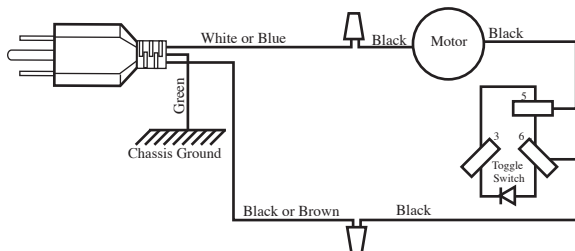
Wiring Diagram for Stainless Steel Top Housing (2nd generation & older units)
