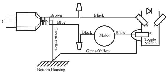
Wiring Diagram for Plastic Top Housing (2nd generation & older units)
