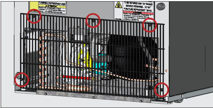
Fig. 1. CVM-11/13 rear grill screw locations. Your application may differ.
