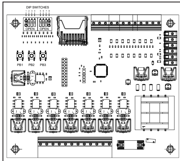
Fig. 67 - Circuit Board
