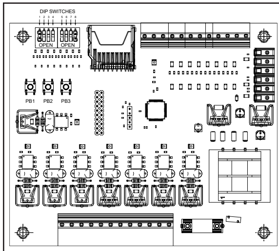
Fig. 28 - Circuit Board
