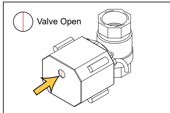
Fig. 63 - Valve position sight window open
