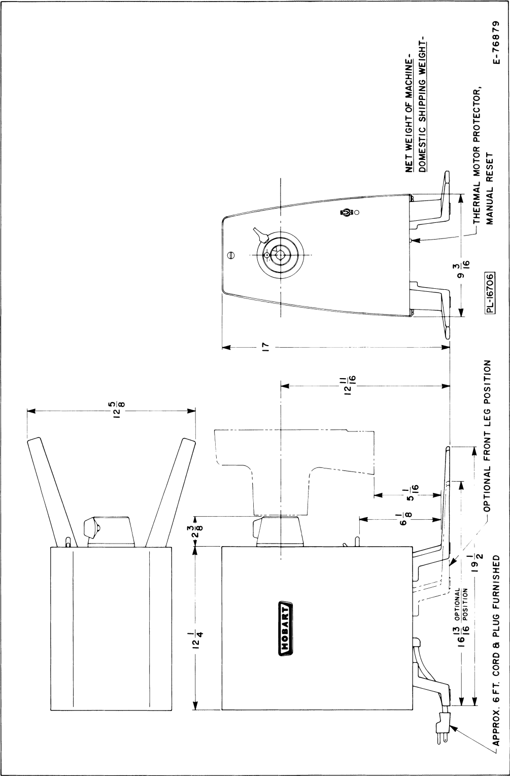
INSTALLATION DIAGRAM
