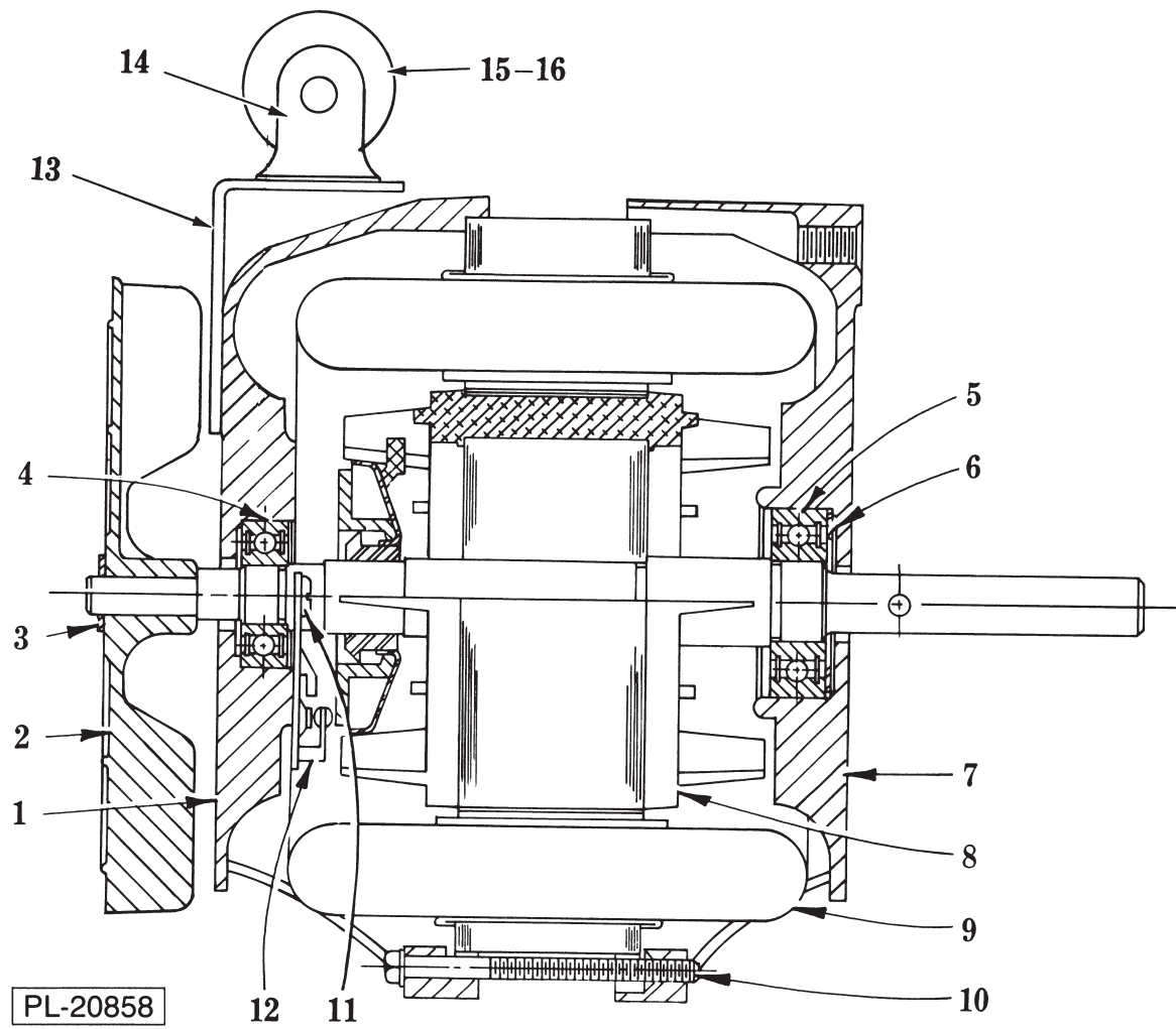
MOTOR UNIT
