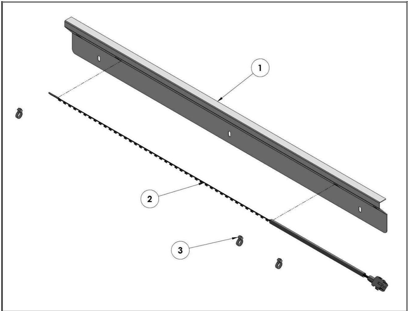
LED ASSEMBLY - TOP PARTS LIST
