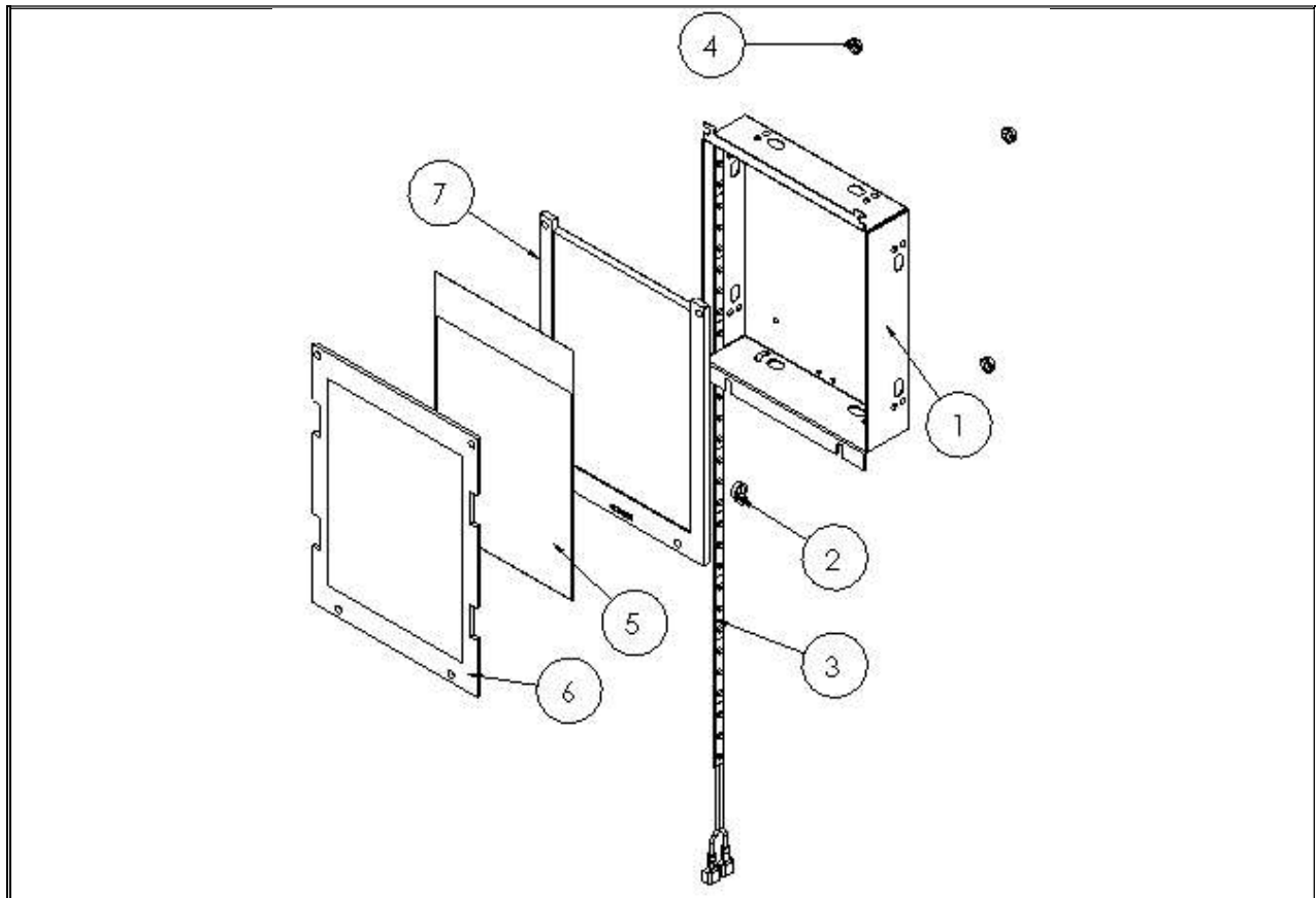
POINT-OF-PURCHASE LED ASSEMBLY 12VDC PARTS LIST
