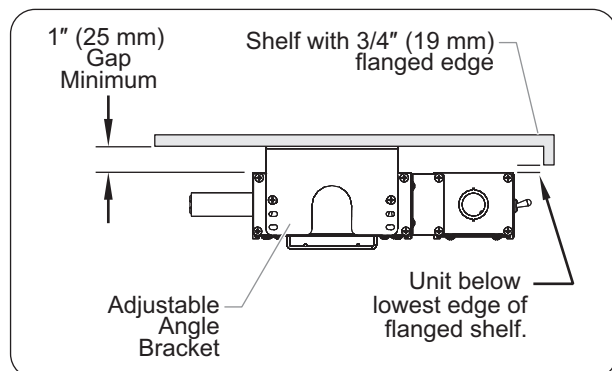
Figure 11. Flanged Shelf Installation
