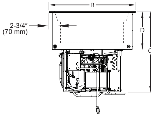
Side View (Model CWB-6)
