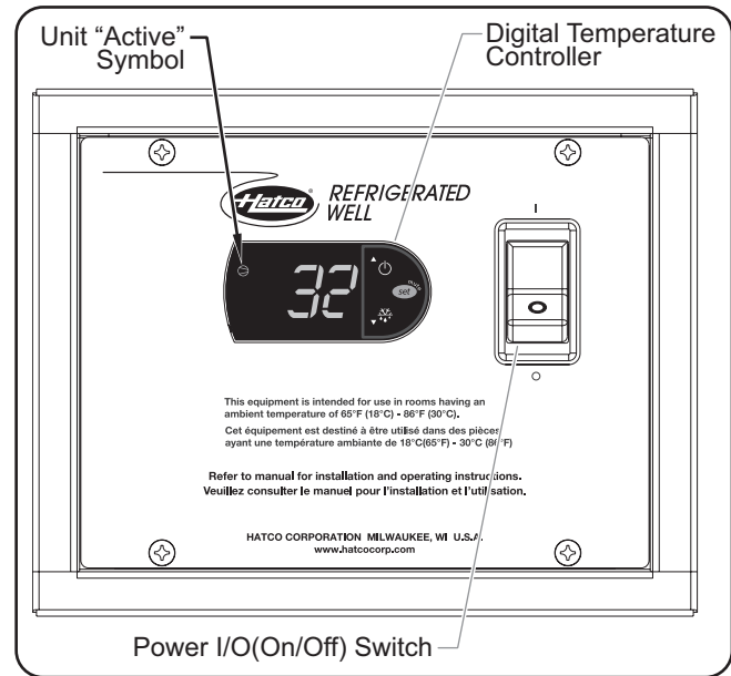
CWB Series Control Box
