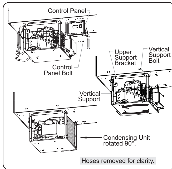
Rotating the Condensing Unit
