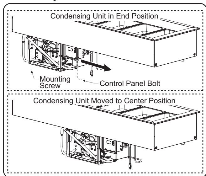
Moving a CWB-5 Model Condensing Unit
