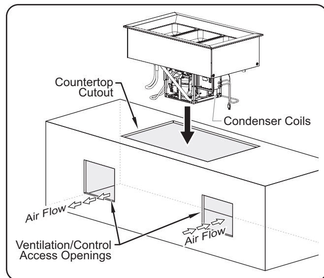
Installing a CWB-3 Model
