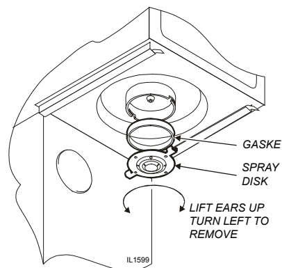
Fig. 8 Cleaning
