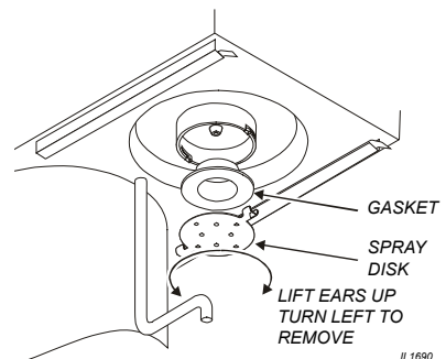
Fig. 8 Cleaning
