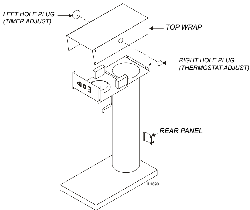
Fig. 8 Access Panels
