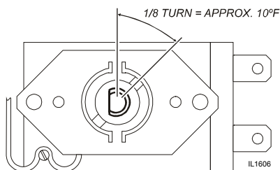
Fig. 10 Adjust Thermostat
