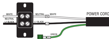
120V 2 WIRE + GROUND
