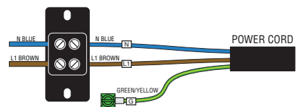
220-240V 2 WIRE + GROUND
